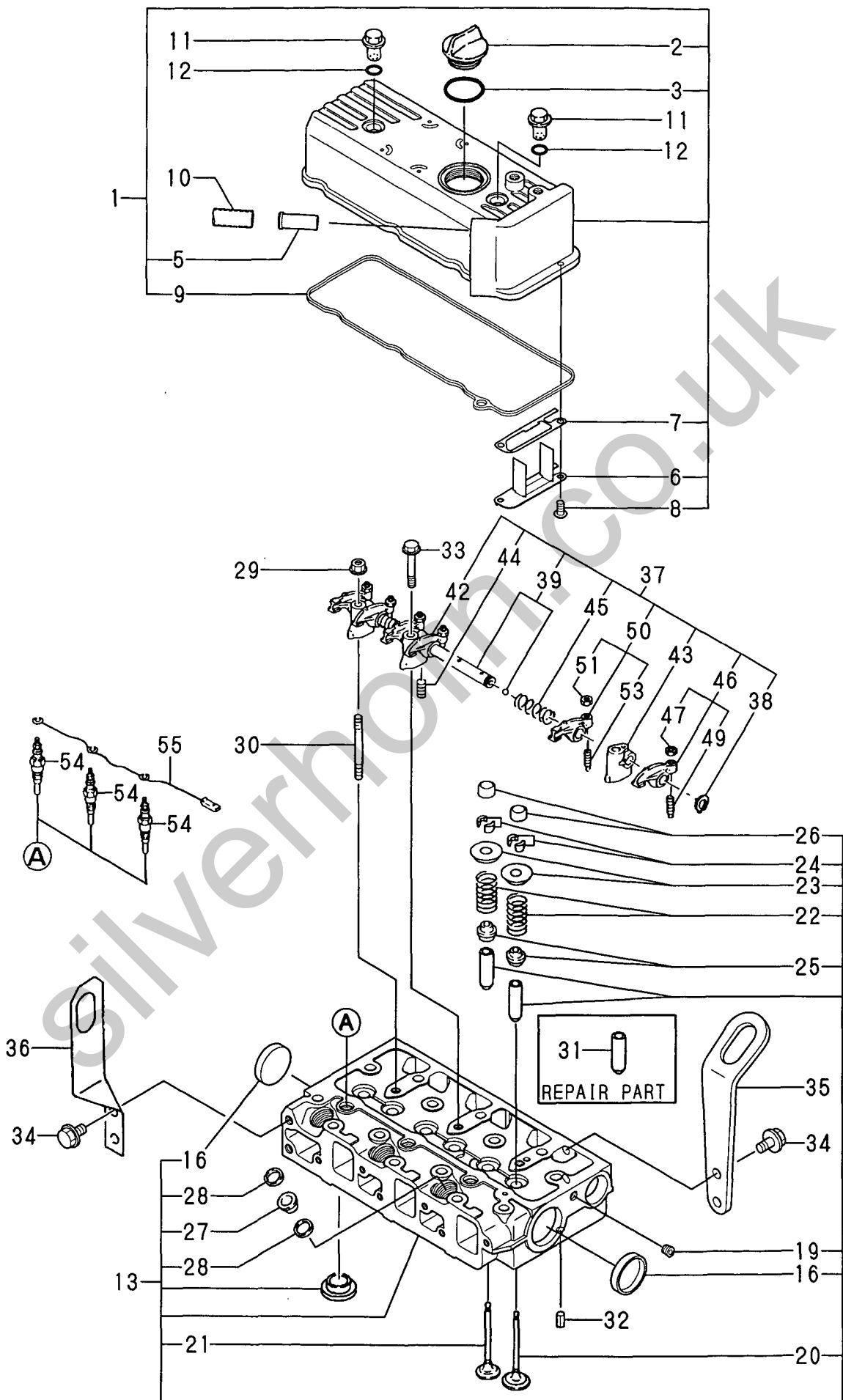
Fig. 4 CYLINDER HEAD & BONNET
