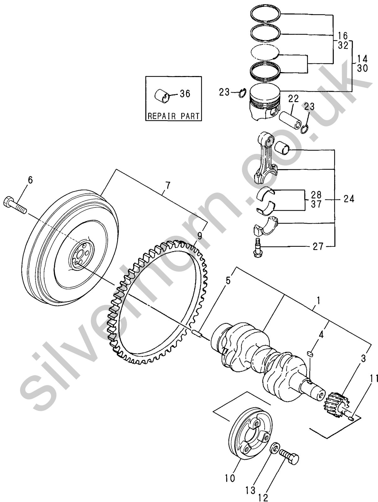
Fig. 7 CRANKSHAFT & PISTON
