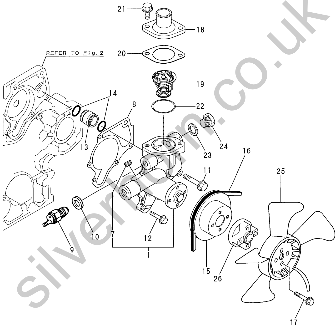
Fig. 9 COOLING WATER SYSTEM
