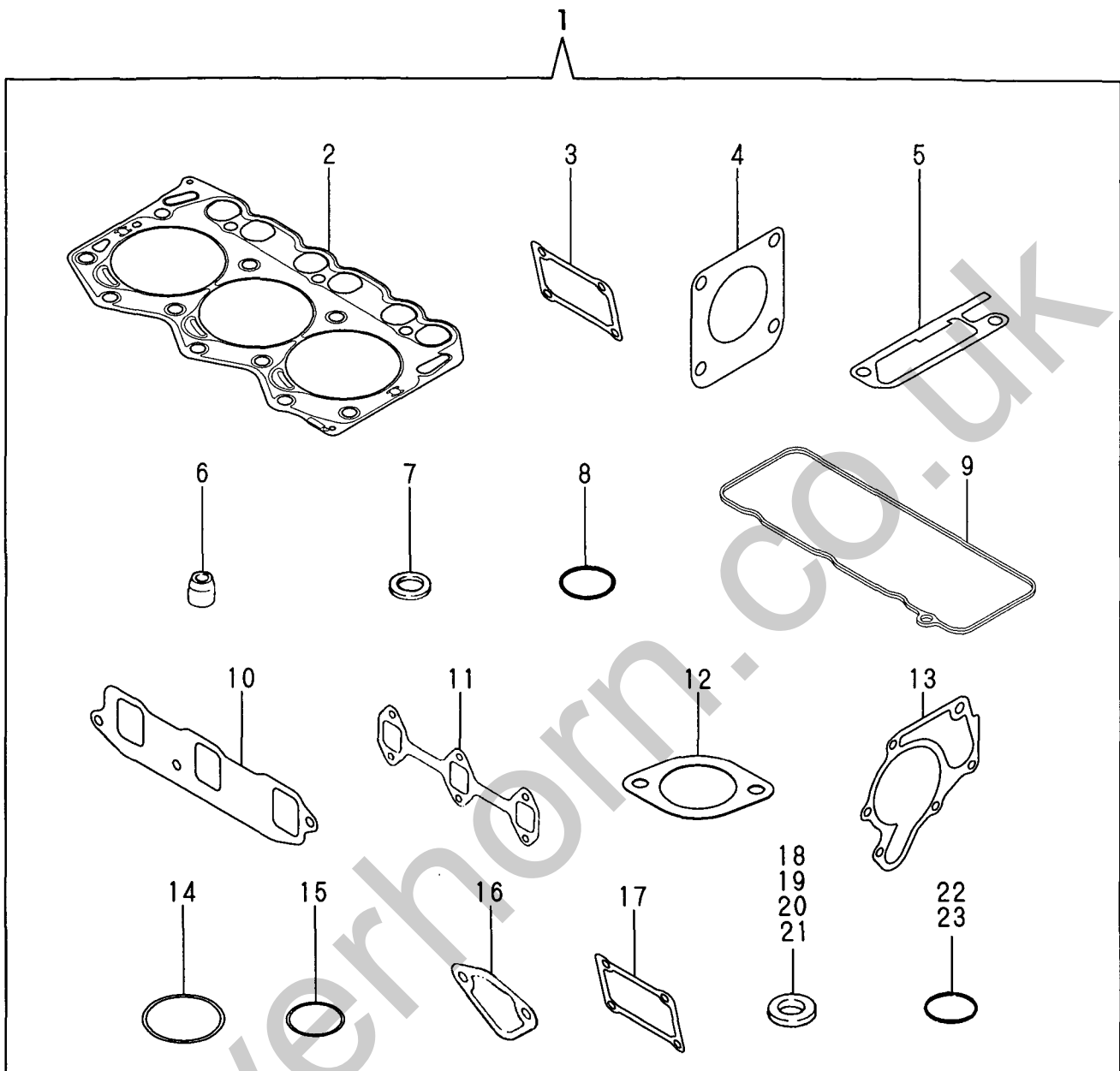
Fig. 15 GASKET SET (OPTIONAL) & TOOL
