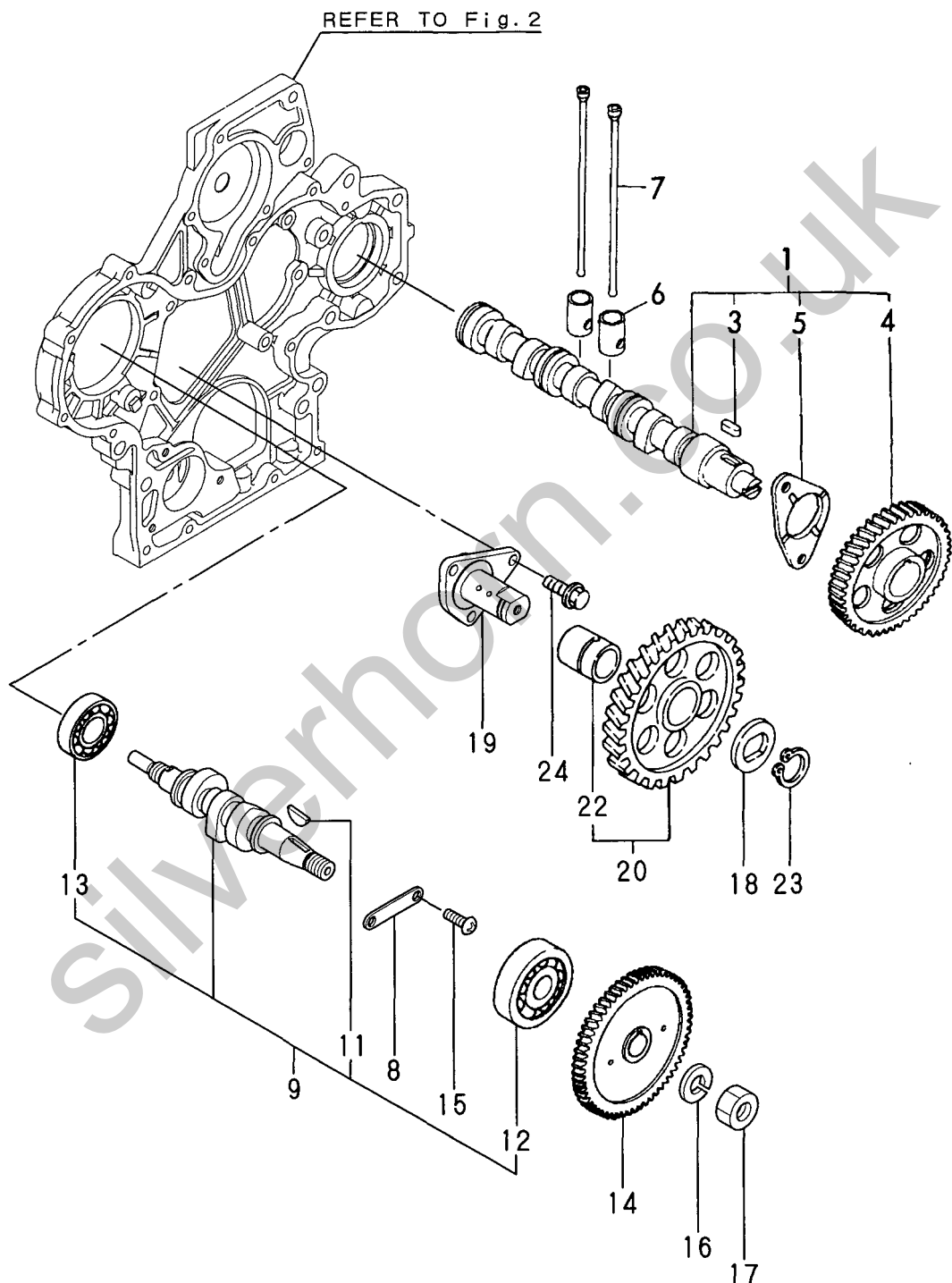
Fig. 6 CAMSHAFT & DRIVING GEAR
