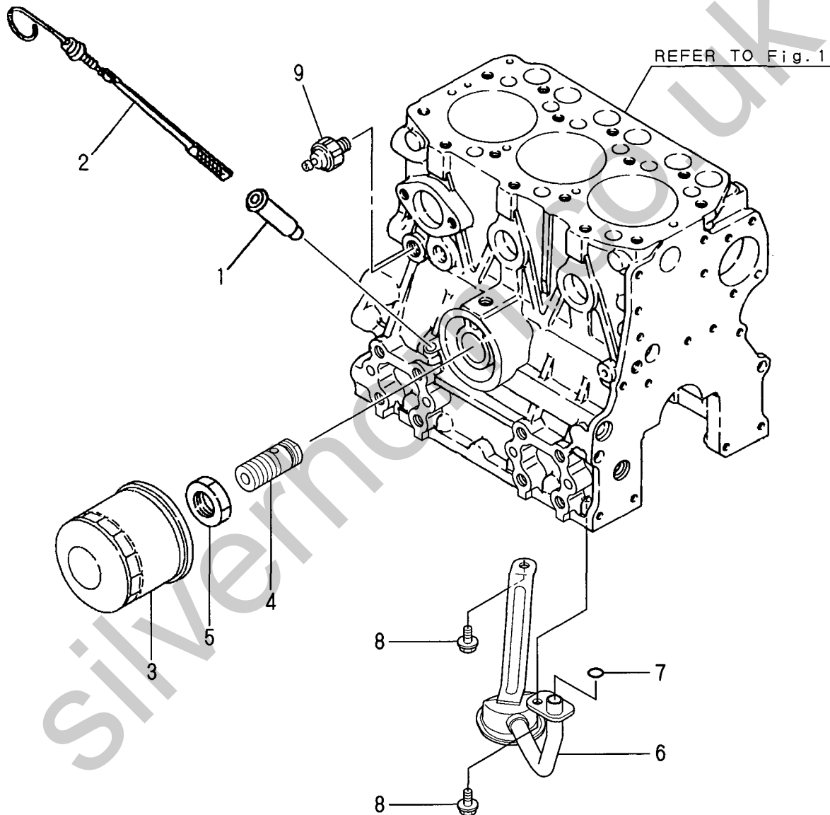
Fig. 8 LUB. OIL SYSTEM
