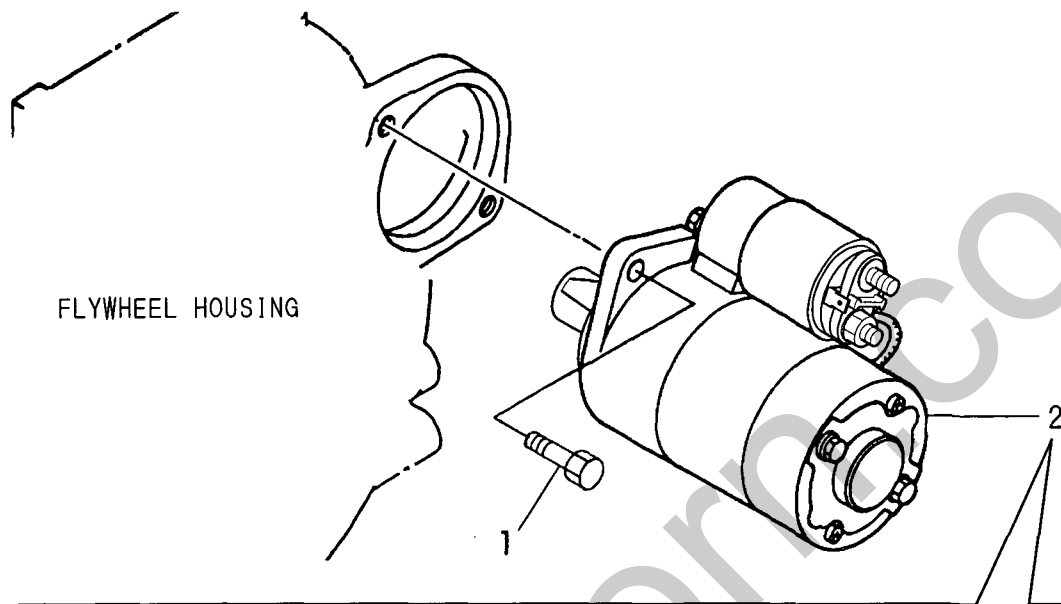
Fig. 13 STARTING MOTOR
