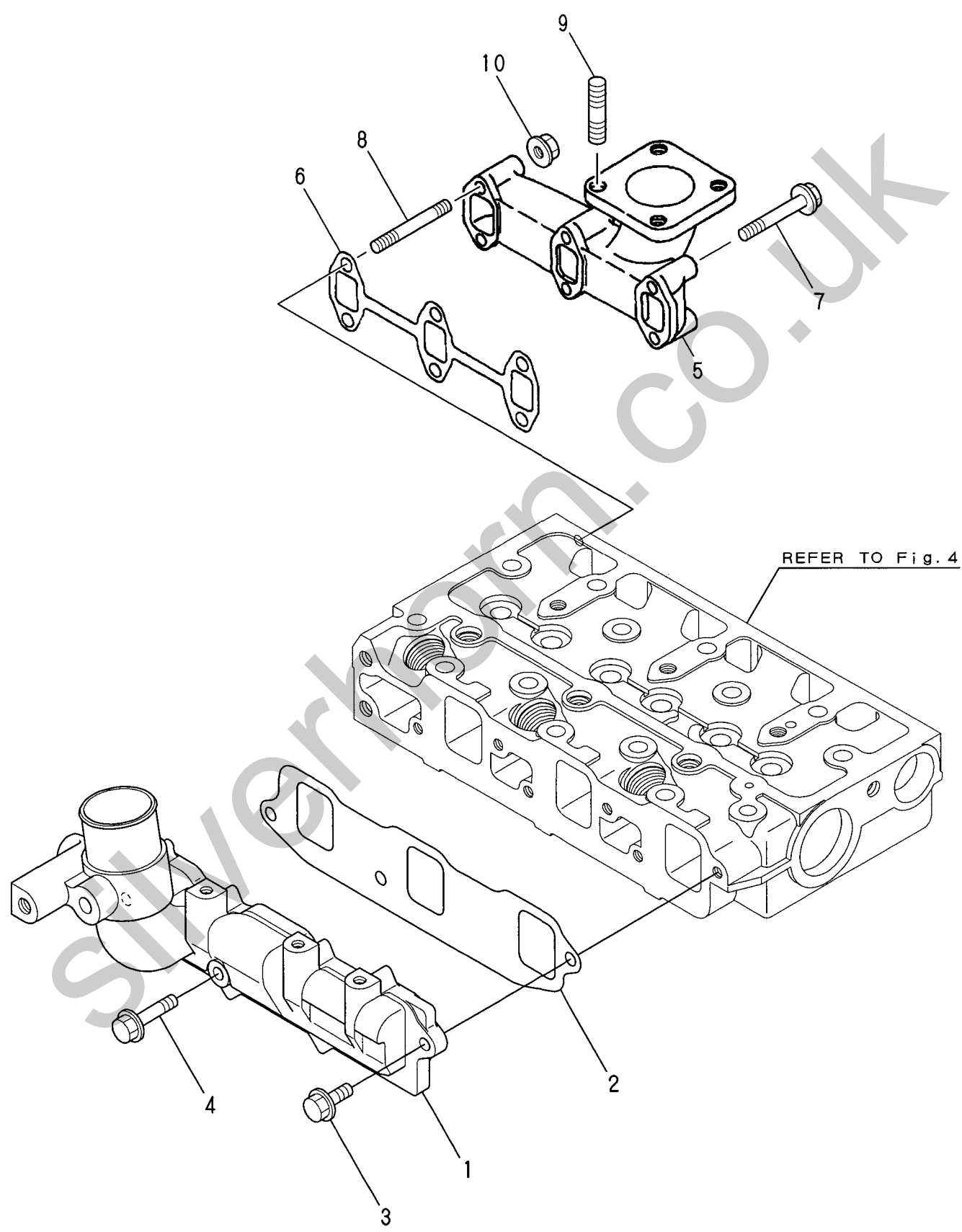
Fig. 5 SUCTION & EXHAUST MANIFOLD
