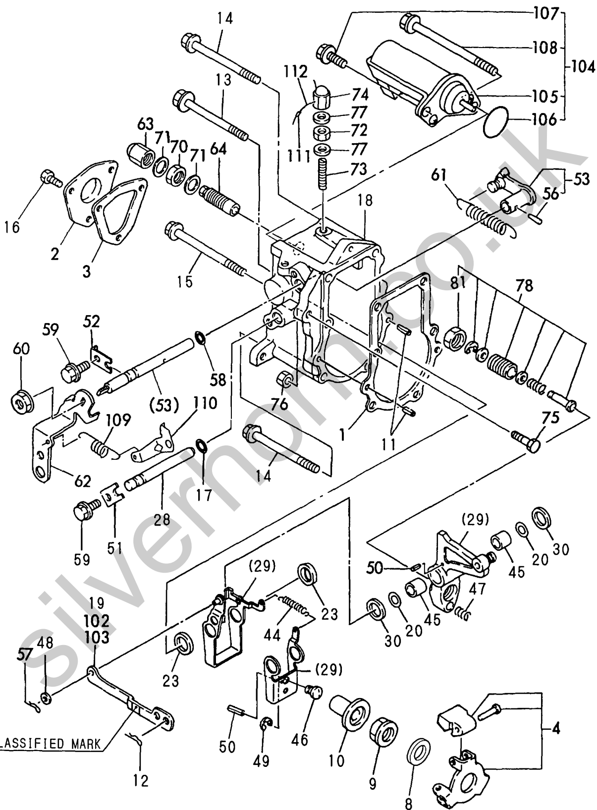
Fig. 12 GOVERNOR
