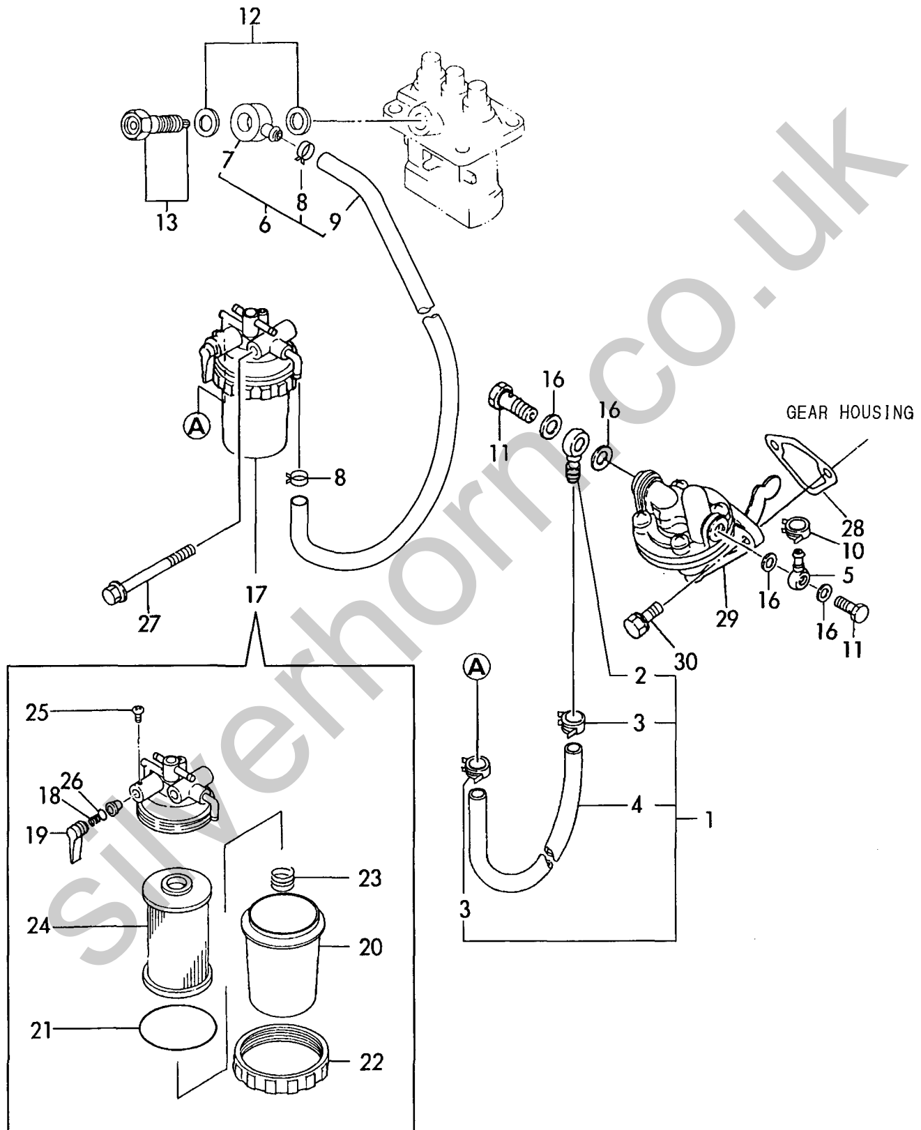
Fig. 11 FUEL PIPE
